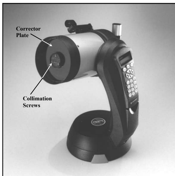
Figure 8-1 The three collimation screws are located on the secondary mirror holder in the center of the corrector plate.
